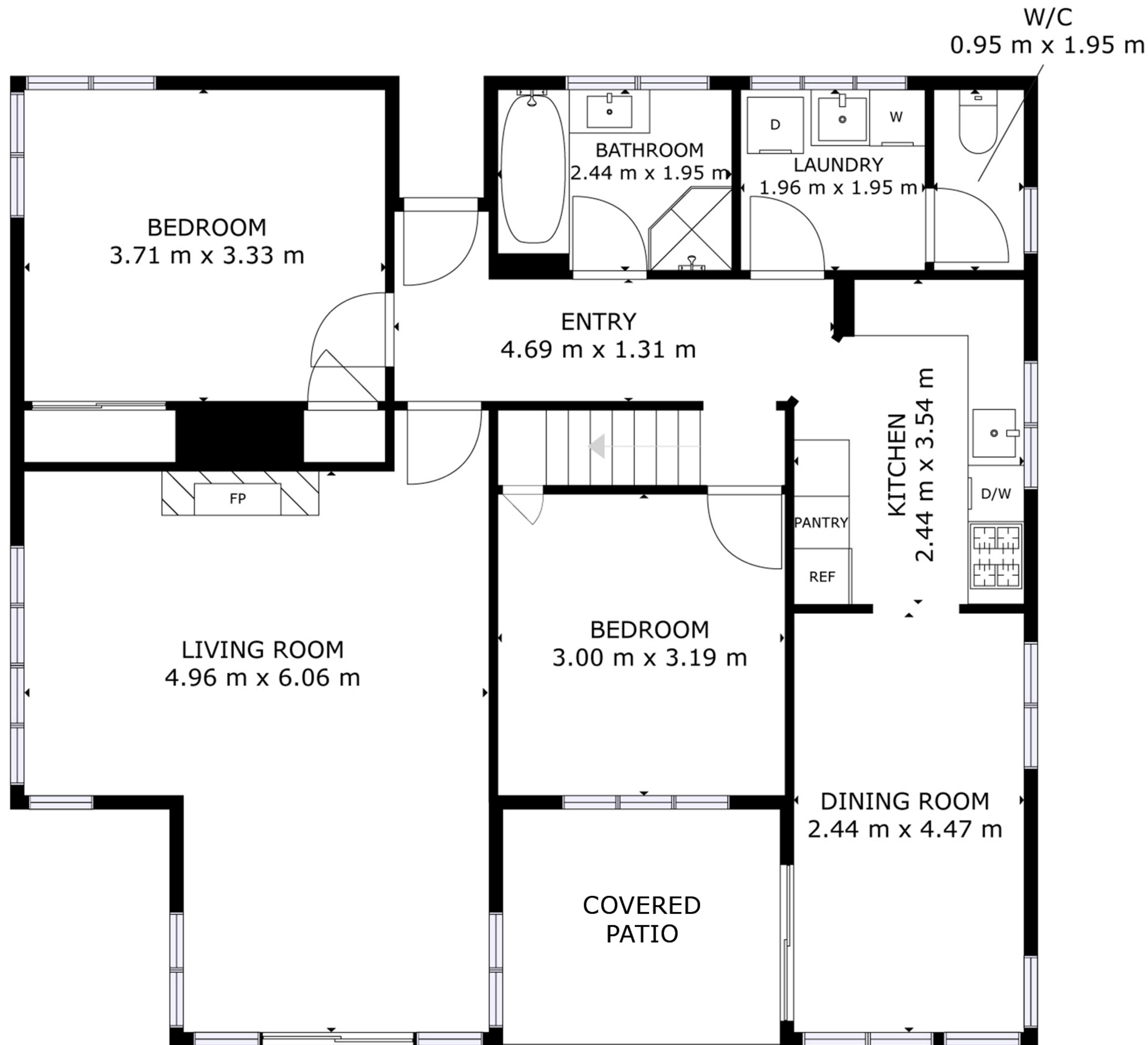
GROUND FLOOR
